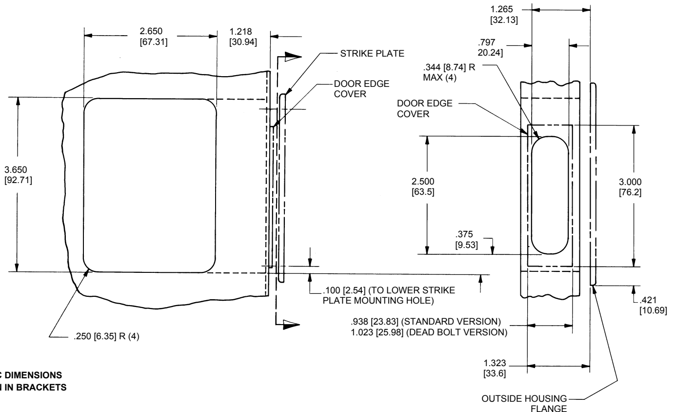
Suggested Door Cut-Out For Latch
