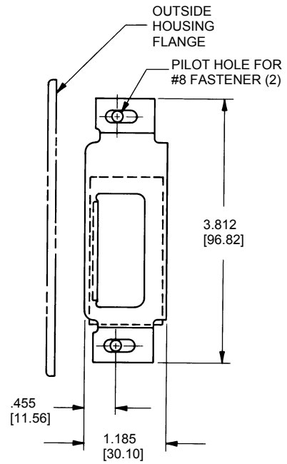
Stamped Steel Strike Plate For Dead Bolt Version
